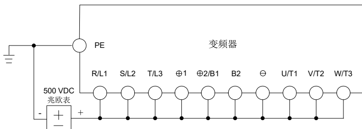
图8-1 E5-H-4T0.75GX~E5-H-4T15GX主回路绝缘测试 E5-P-4T1.5X~E5-P-4T18.5X主回路绝缘测试 E5-A-4T15X~E5-A-4T18.5X主回路绝缘测试
